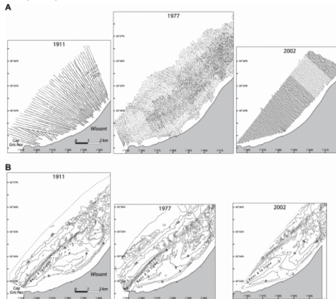
Fig. 3 – (A) Location of depth soundings in the Bay of Wissant for the 1911, 1977, and 2002 surveys ; (B) Bathymetry of the Bay of Wissant in 1911, 1977, and 2002.
