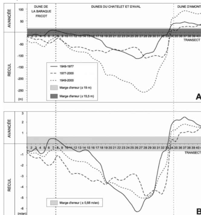
Fig. 6 – A) : coastline evolution in the Bay of Wissant from 1949 to 2000 ; B) : Mean rates of coastline evolution for the periods 1949-1977, 1977-2000, and 1949-2000.
