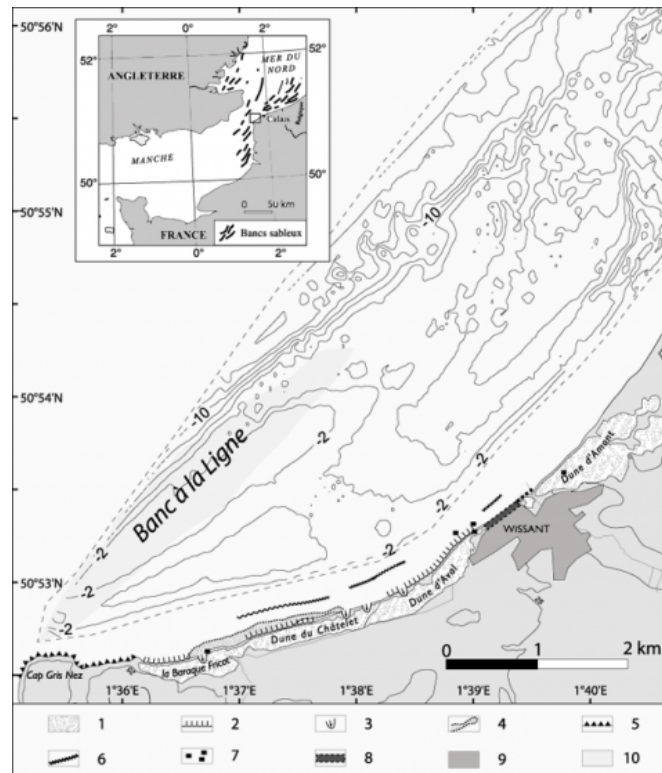
Fig. 1 – Location of the study area (depth contours correspond to the 2002 bathymetry ; terrestrial part of the map, modified after Messence and Cohen, 2002).
